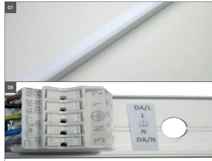
(07) Front part has to be flush mounted. Push it hard to mounting plate till you can hear the „Click“. Please check that front part is fixed securely.
