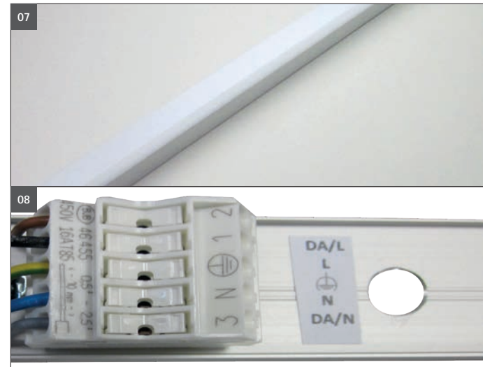
07 (07) Front part has to be flush mounted. Push it hard to mounting plate till you can hear the „Click“. Please check that front part is fixed securely.
