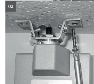
Assembly with ceiling rose
