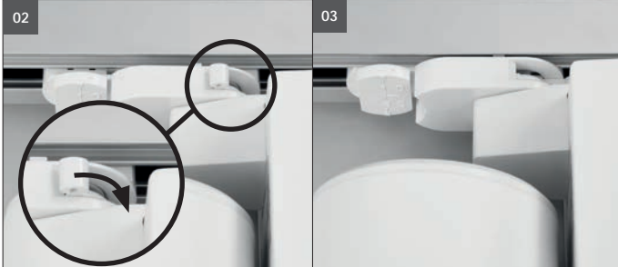
Insertion and locking of 3-phase universal adapters.
